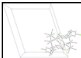
Fig. 2. A pair of molecules is linked into a dimer by intermolecular hydrogen bonds (dashed lines).
